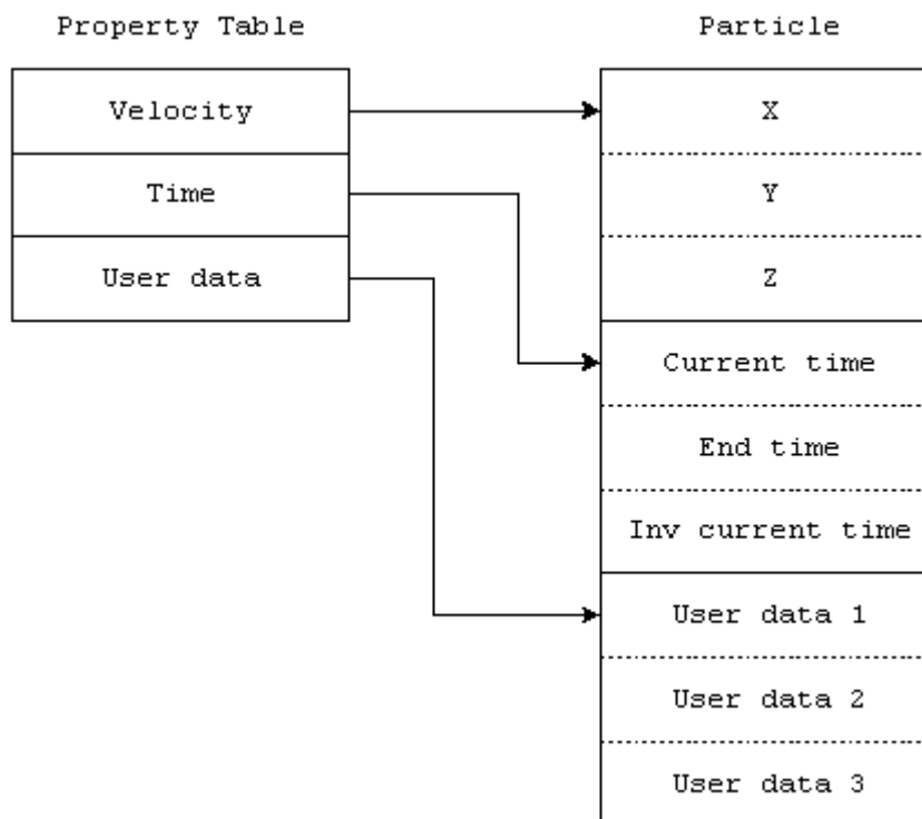
Fig 2. Example of a property table defining a particle.
