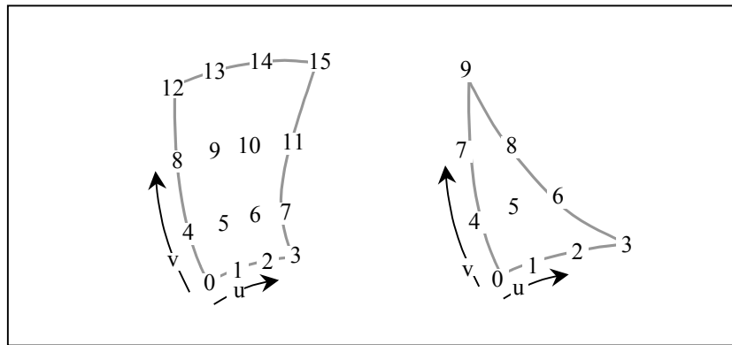
Order of control points for a patch
