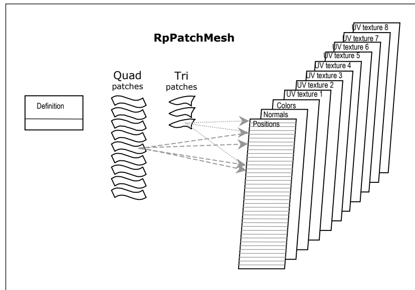
A more literal representation of RpPatchMesh
