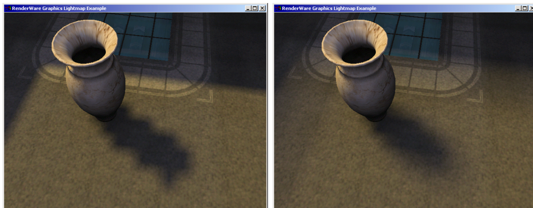
The shadow in front of the vase on the left reveals the texels of the light map. The jittered version to the right tends to hide them.
