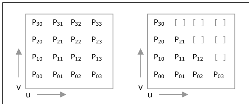
Positions of control point numbers for quad and tri patches in an RtBezierMatrix
