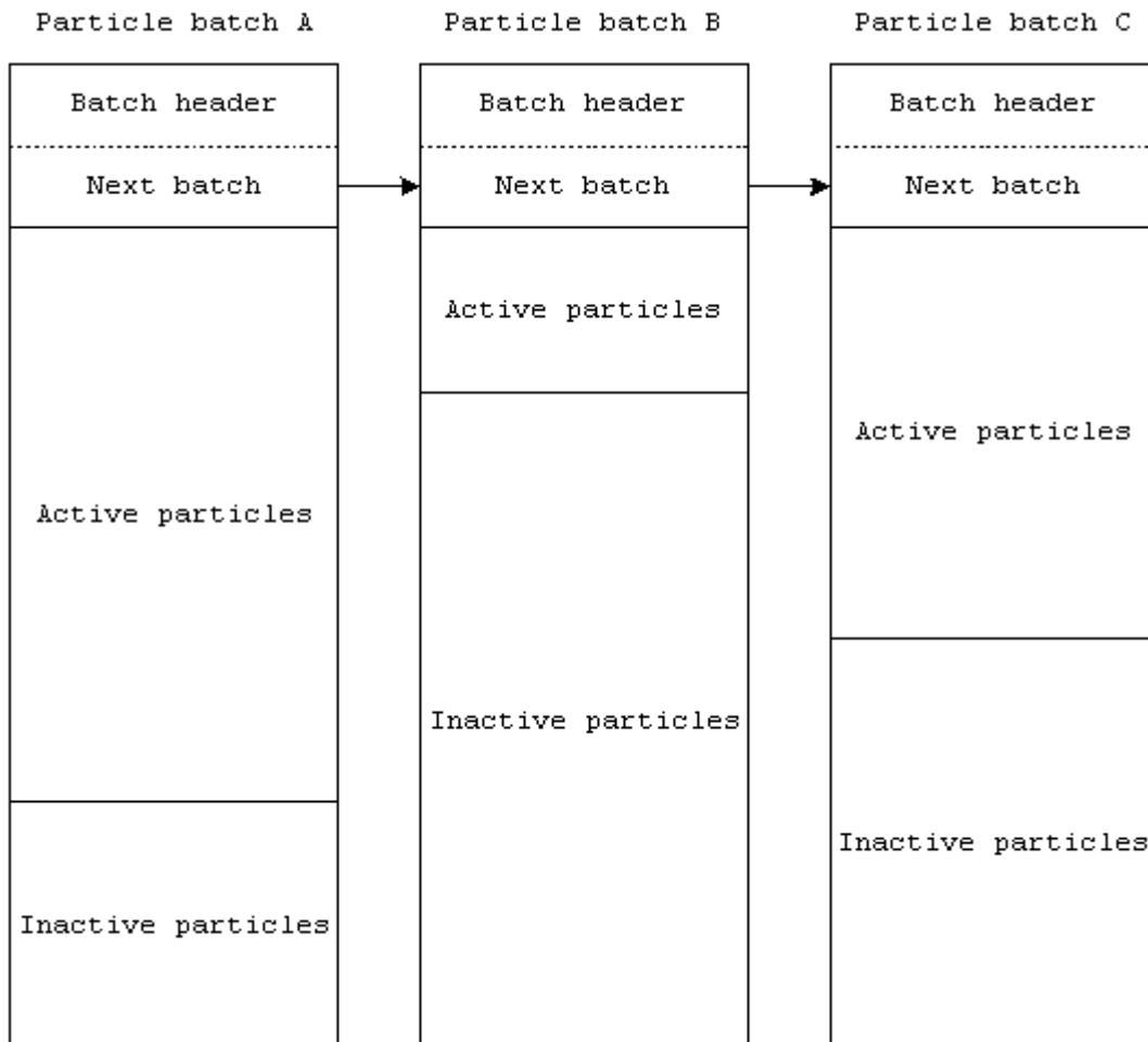
Fig 1. Example of a list of particle batches, each with different number of active particles.
