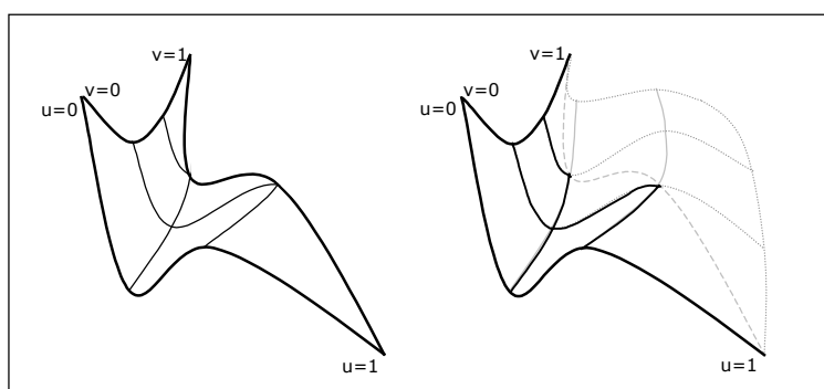
A quad patch can retain coordinates coincident with a tri patch
