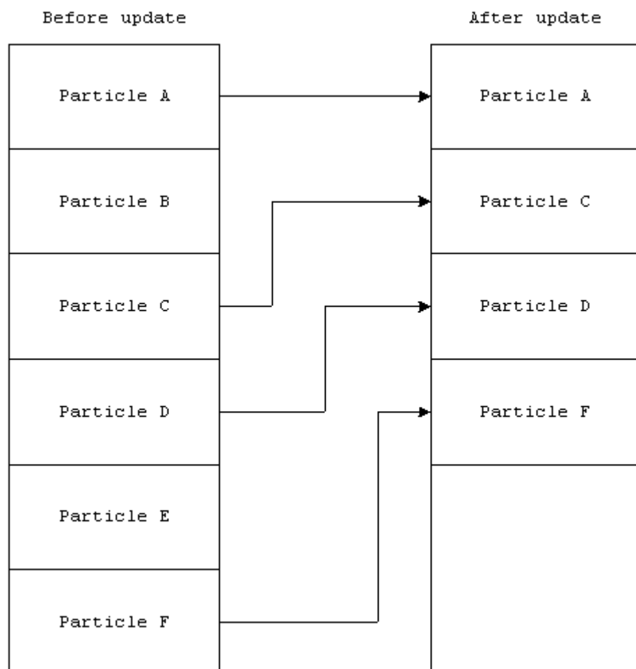
Fig 3. Example of particle removal. Particle B and E are removed by being overwritten by other remaining active particles.
