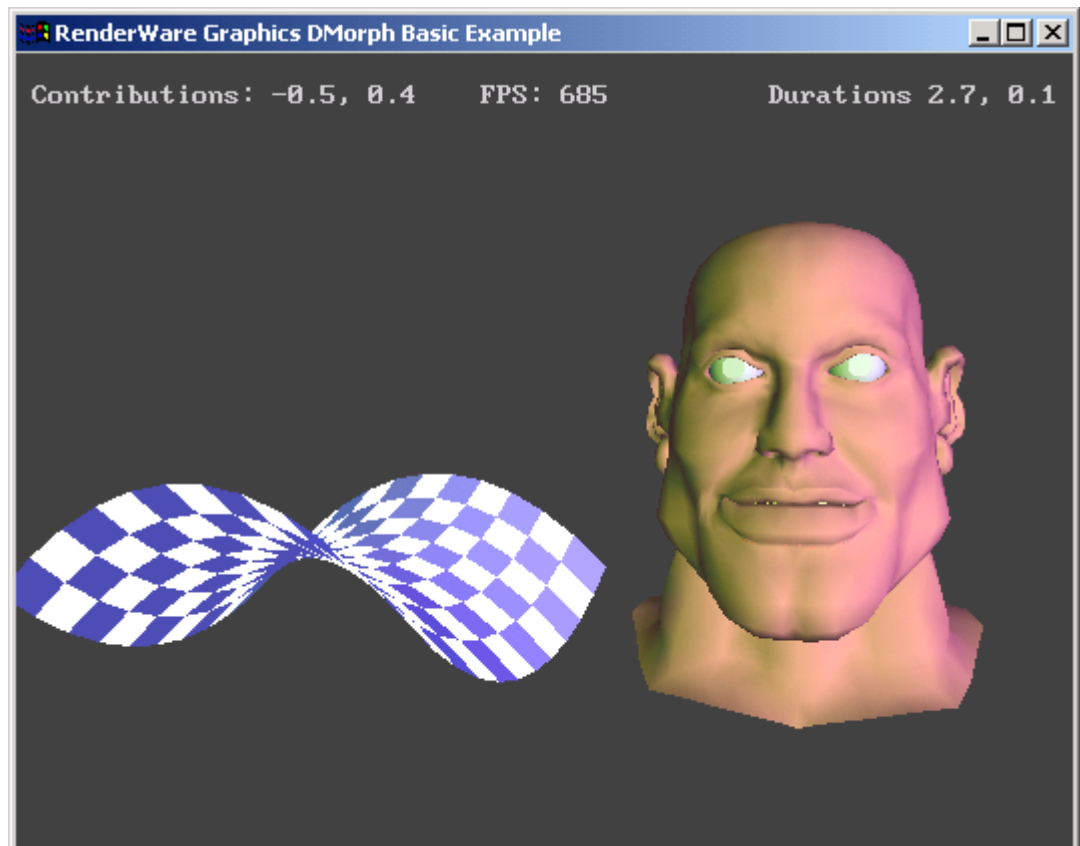
DMorph Example
