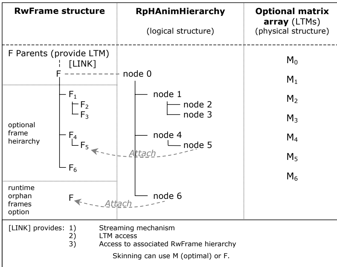
Hierarchy Overview
